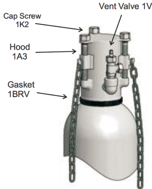
Chlorine Cylinder DOT 3AA480
